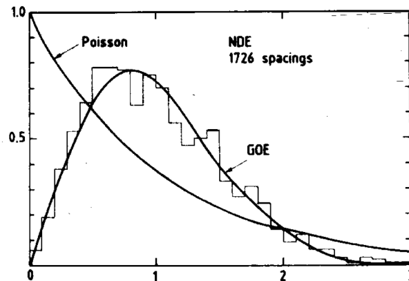
FIGURE 1 – Nearest neighbor spacing distribution for the “Nuclear Data Ensemble” comprising 1726 spacings (histogram) versus s = S/D with D the mean level spacing and S the actual spacing. For comparison, the Wigner surmise labelled GOE is shown (don’t mind about the curve labelled Poisson).
